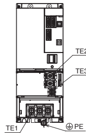
Terminal diagram (with front cover open)
